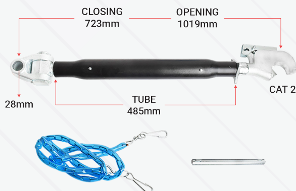
HEAVY DUTY TOP LINK KH282485 New Holland Series
