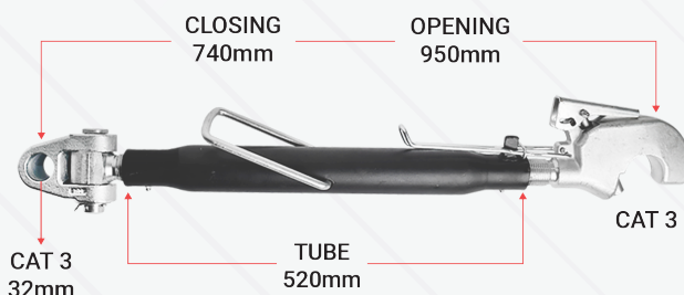
HEAVY DUTY TOP LINK KH33520
