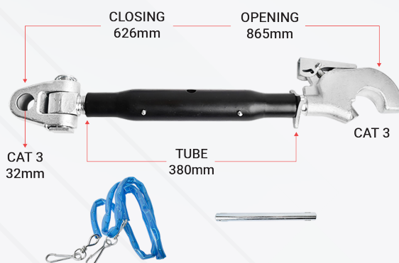
HEAVY DUTY TOP LINK KH33380
