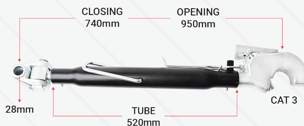
HEAVY DUTY TOP LINK
