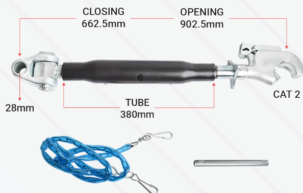
HEAVY DUTY TOP LINK KH282380 New Holland Series
