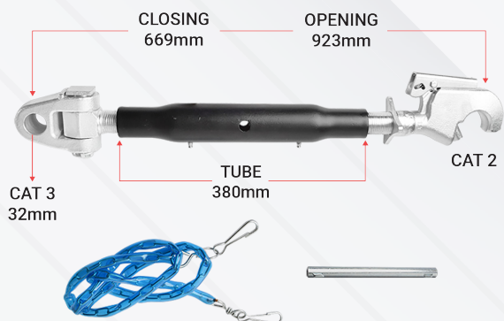
HEAVY DUTY TOP LINK KH32380
