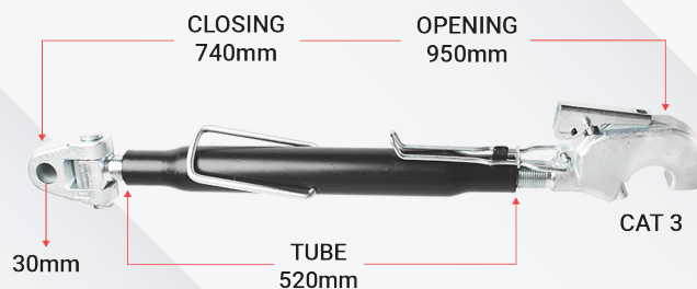
HEAVY DUTY TOP LINK KH303520
