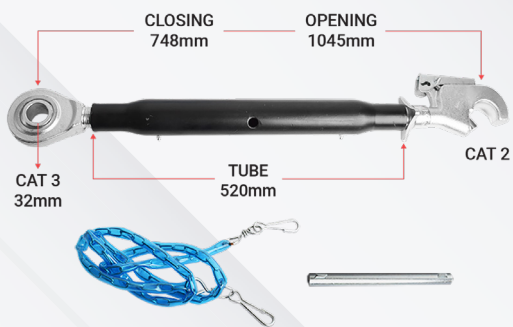
HEAVY DUTY TOP LINK BH32520
