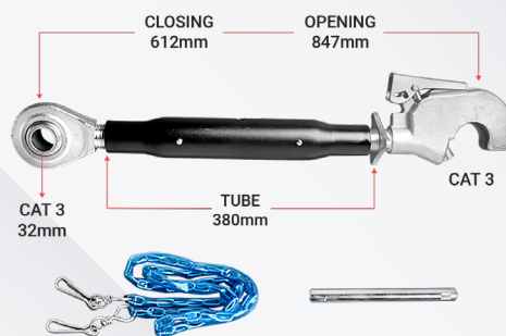
HEAVY DUTY TOP LINK BH33380
