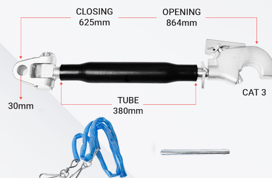
HEAVY DUTY TOP LINK
