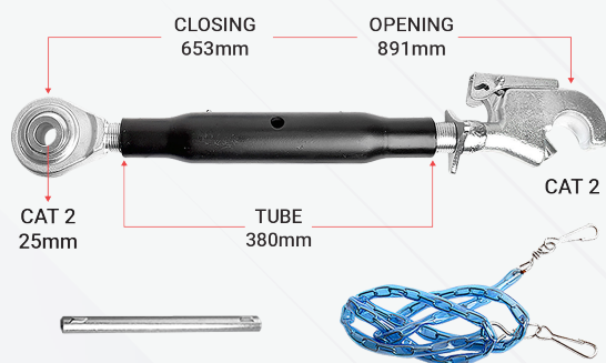
HEAVY DUTY TOP LINK BH22380
