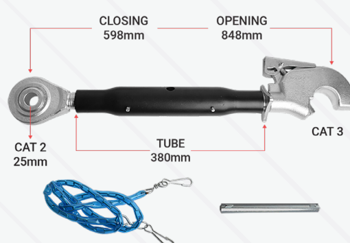
HEAVY DUTY TOP LINK BH23380
