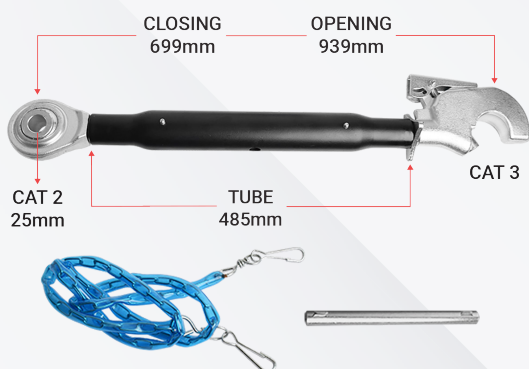
HEAVY DUTY TOP LINK BH23485
