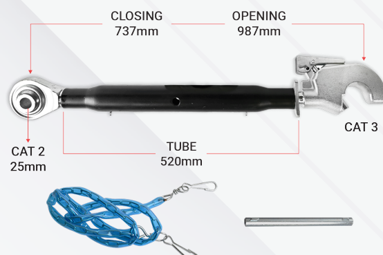
HEAVY DUTY TOP LINK BH23520
