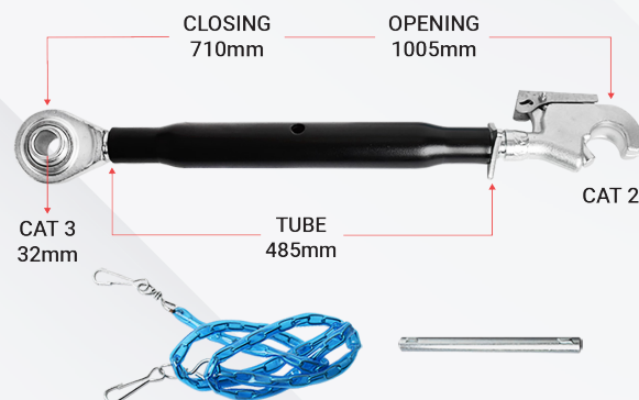
HEAVY DUTY TOP LINK BH32485
