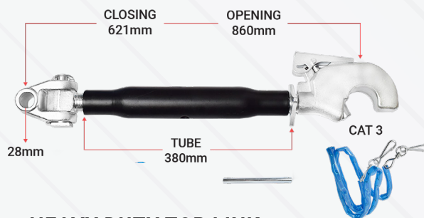
HEAVY DUTY TOP LINK
