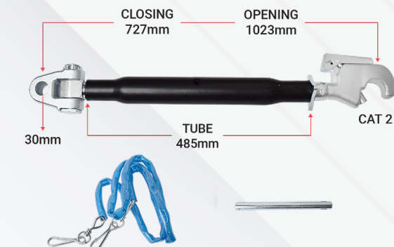
HEAVY DUTY TOP LINK
