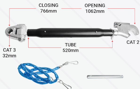
HEAVY DUTY TOP LINK KH32520
