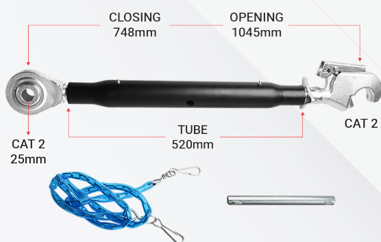
HEAVY DUTY TOP LINK BH22520
