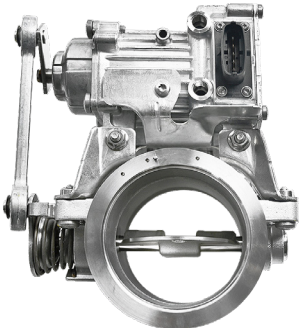
ENGINE EXHAUST BRAKE VALVE 401006 | OE Ref: 47669650 NEF 4 Cylinder engine New Holland T5 Case IH Vestrum Series
