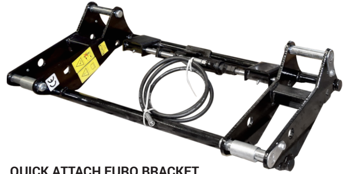
QUICK ATTACH EURO BRACKET CARRIER FRAME HYDRAULIC LOCKING 55802
