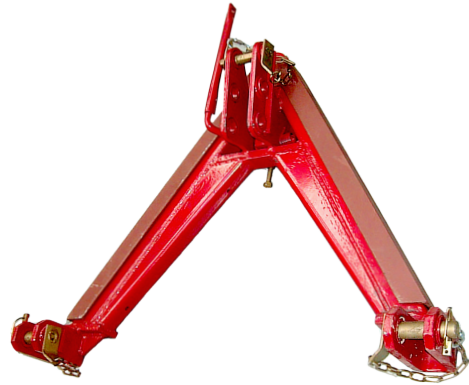
REAR LINKAGE QUICK HITCH KIT CAT 2 51228K | OE Ref: S.23464
