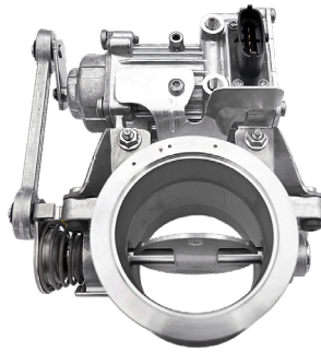
ENGINE EXHAUST BRAKE VALVE 401008 | OE Ref: 87547824 NEF 4 Cylinder Engine New Holland T6 Case IH Maxxum Series
