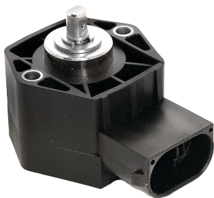
POSITION SENSOR 65014 | OE Ref: 34253500 Deutz Agrottron Series
