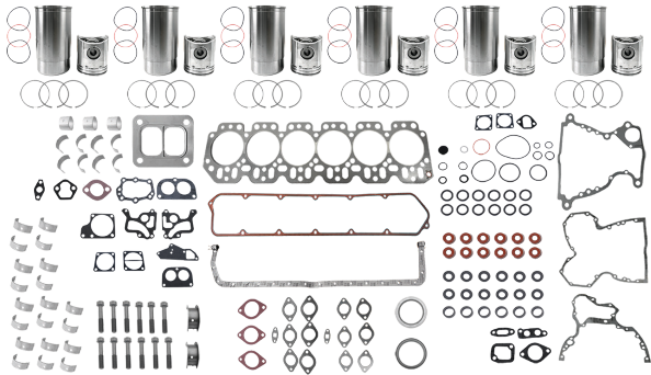
MAXIFORCE ENGINE KIT 501204 | OE Ref: AR67942
