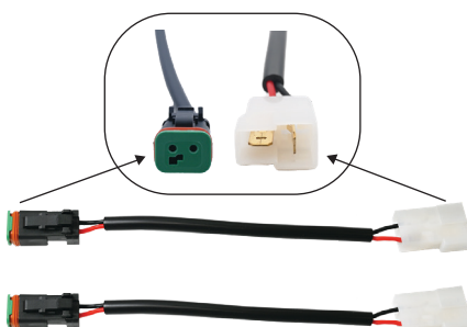
ADAPTOR CABLE DT 2 PIN 6.3 SOCKET
