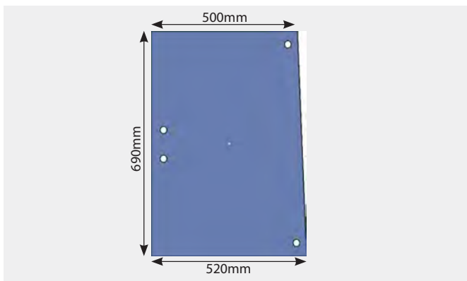
D6616 Glass 600 Side Window Left Hand & Right Hand
