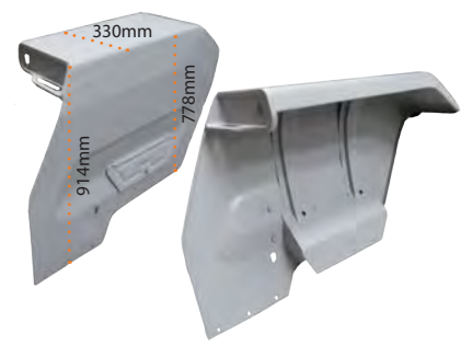
63300 Mudguard 165 178 PAIR Square 31' with Toolbox
