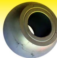
Lower Link Ball Cat 3/3 ID 37.5mm OD63.5mm
