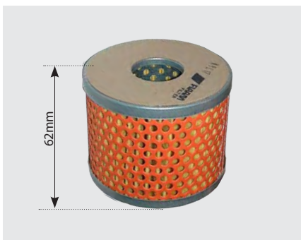
1883318 Massey Ferguson Power Steering Filter Old Type OE Ref: 1883318M1
