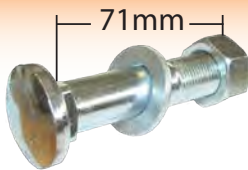
1330 Rim to Disc Bolt Ford c/o Nut & Washer (5/8 UNF x 71mm long) Square Shoulder
