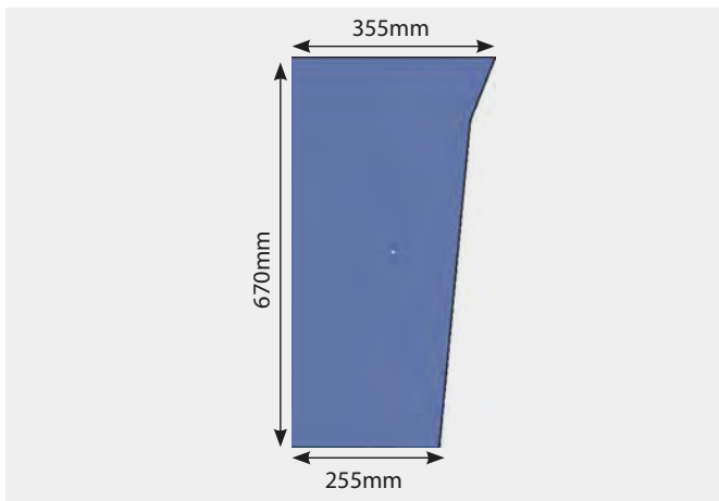
D6903 Glass 300 Right Hand Lower Front - No Holes
