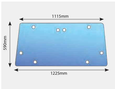
2227 Glass 300 Top Rear Window Black Cab OE Ref: 3476182M1
