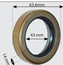
825740 Timing Cover Seal 20D (WRH11) OE Ref: 108735C1
