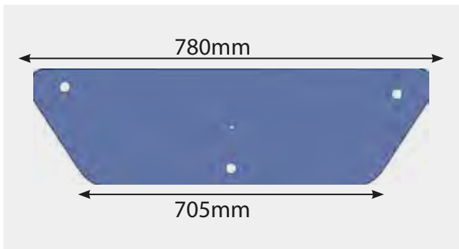
2228 Glass 300 Bottom Rear Window
