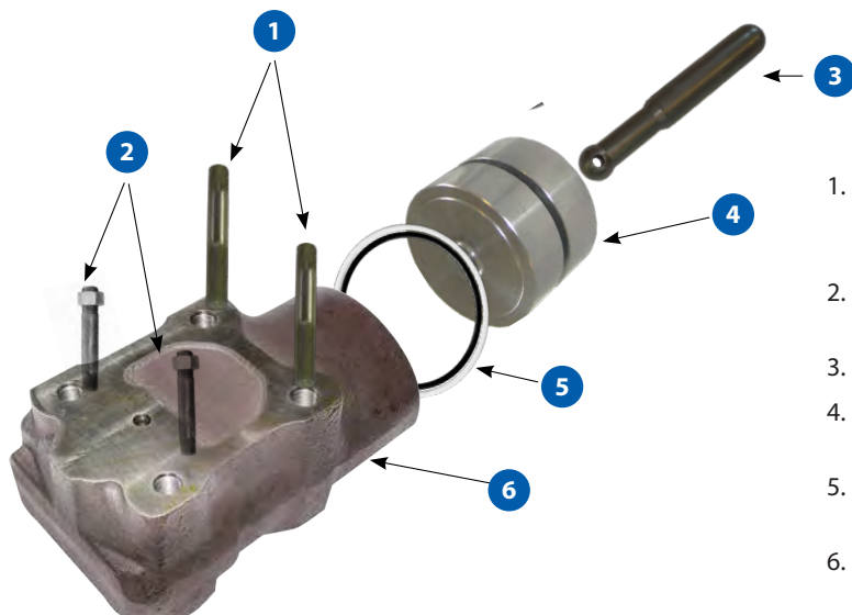
6574 Massey Ferguson Tee-piece for Spool Valve 300
