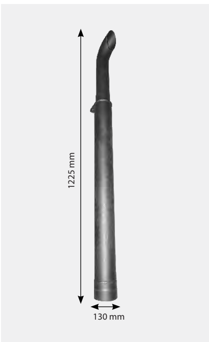
61934 Massey Ferguson Exhaust 6190
