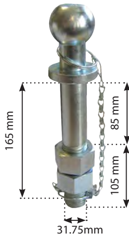
1403 Hitch Pin and Ball 1 1/4"
