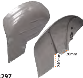
63297 Mudguard 35X 9 1/2" PAIR Red c/w Weld Brkt 61625 is Mudguard Light Bracket 35X
