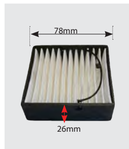
680020 30 Micron Pre Fuel Filter 5400 6400 7400 Series OE Ref: F916200060010
