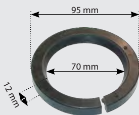
825208 Crankshaft Seal TVO Rear OE Ref: 825208M1
