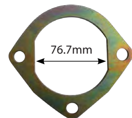
Massey Ferguson PTO Retainer Plate Early 35 135
