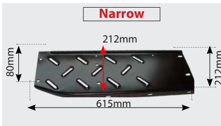
61465 Foot Board 135 Right Hand - Narrow 8 1/2"
