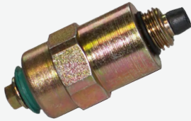
1992 Solenoid Diesel Stop OE Ref: 9986316
