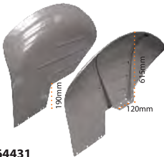
64431 Mudguard 35X 7" PAIR Red c/w Weld Bracket 61625 is Mudguard Light Bracket 35X
