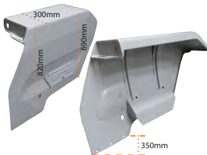
63299 Mudguard 135 & Box PAIR 28' Narrow 10.5' Tool Box Reinforcing Plate is 62542
