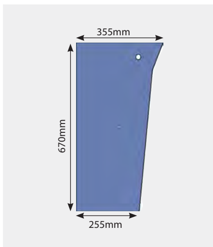
D6902 Glass 300 Left Hand Lower Front + Holes OE Ref: 3475994M1
