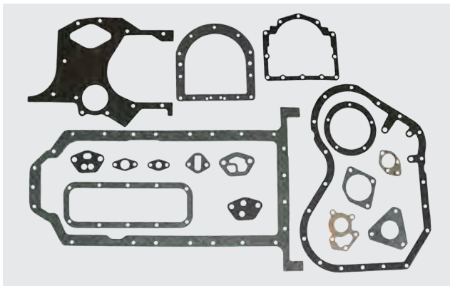
68211 Sump Gasket Set 318
