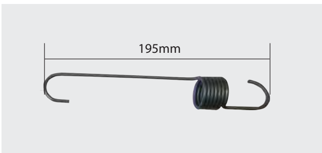
62987 Spring 54s Clutch Pedal Early Type Up To Serial No M342025 OE Ref: 3788068M1
