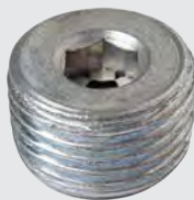
62553 Massey Ferguson Water Pump Plug 65 135 285 Series Size: 1/2" - 14 OE Ref: 2431154
