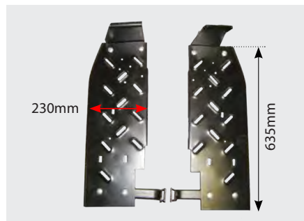
62828 Foot Step 135 240 Pair c/o Brackets
