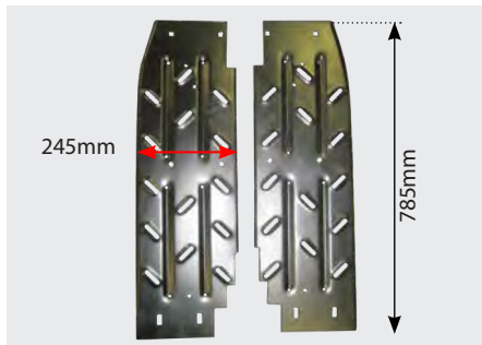
62826 Foot Step 188 265 285 290 Pair Length 31" Width 10"
