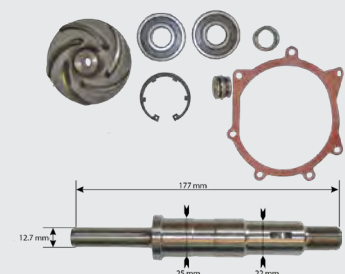
U7LW0015 Water Pump Repair Kit
