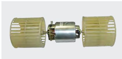
62780 Fan Cab Blower 3000 6100 5400 6200 8100 Also fits 8200 OE Ref: 3310831M91
