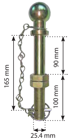
4672 Hitch Ball 7 1/2" x 1" Pin & Chain
