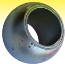
Lower Link Ball 57mm OD 36.5mm ID 44.5 Width
