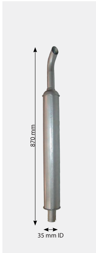
61328 Exhaust 20D 20TVO Horizontal 61298 – Clamp
