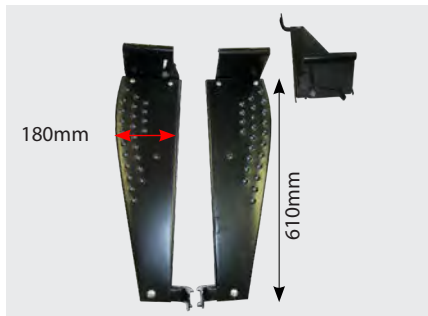
62824 Foot Step 35 Pair w/ Bracket & Bolts
