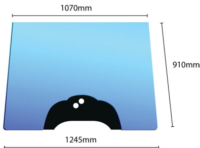
GLASS WINDSCREEN 64734 | OE Ref: 3821747M1 Massey Ferguson 4200 4300 Series | 2 Holes
