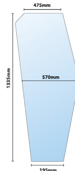
GLASS DOOR RH 7253 | OE Ref: 5125038 1888 - 5 | 10 | 20 Fiat 90 94 Classique Series
