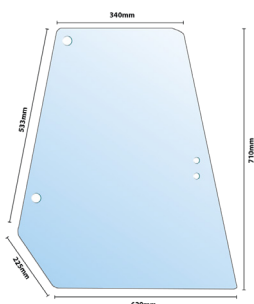
GLASS SIDE 7062 | OE Ref: 5124412 1888 - 5 | 10 | 20 Fiat 90 94 Classique Series | 4 Holes
