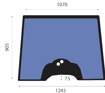
GLASS WINDSCREEN 63188 | OE Ref: 3821746M1 Massey Ferguson 4300 Series | 2 Holes
