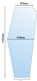
GLASS DOOR LH 7264 | OE Ref: 5124414 1888 - 5 | 10 | 20 Fiat 90 94 Classique Series
