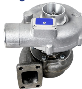
TURBOCHARGER 680342 | OE Ref: F186200090010 Fendt Farmer 300 Series
