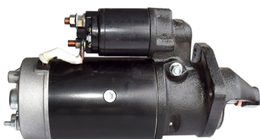
STARTER 780241R | OE Ref: F13590206010 Fendt 102-108 Series
